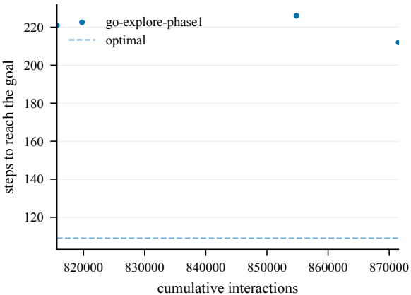
Steps to goal (train) -- ChamberCount8-100@4002
