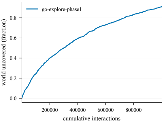
Cumulative coverage -- ChamberCount8-200@4002
