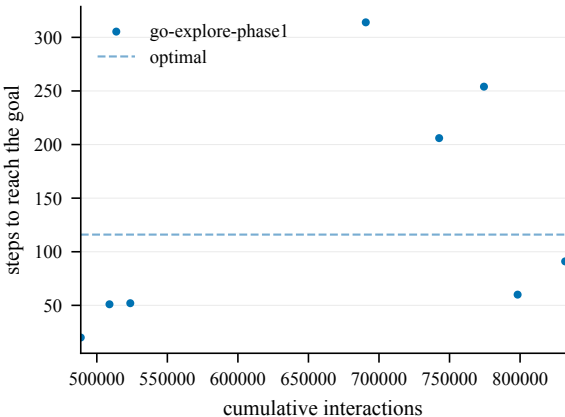
Steps to goal (train) -- Chambers2-100@4000
