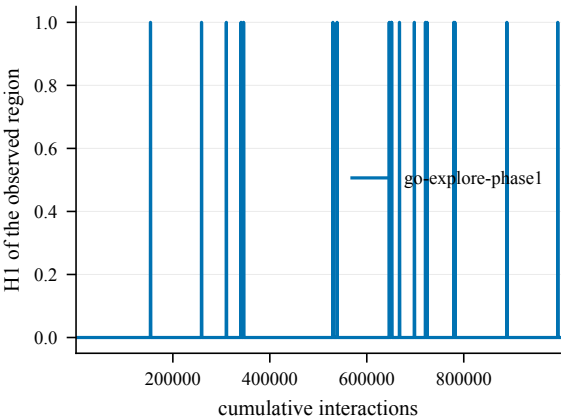
Discovered topology -- Chambers2-100@4001
