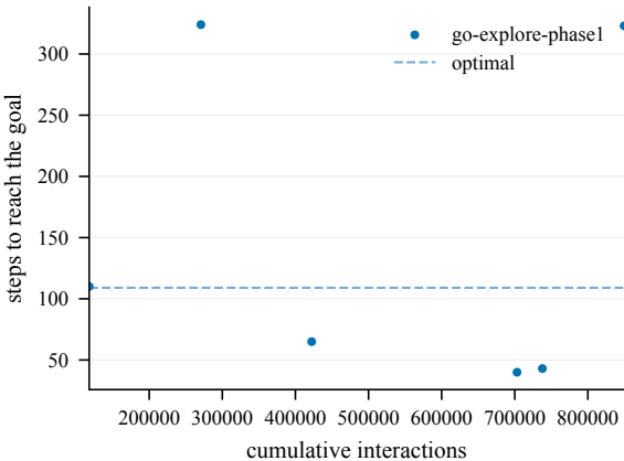
Steps to goal (train) -- Chambers2-100@4001
