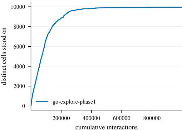
States discovered -- Chambers2-100@4001
