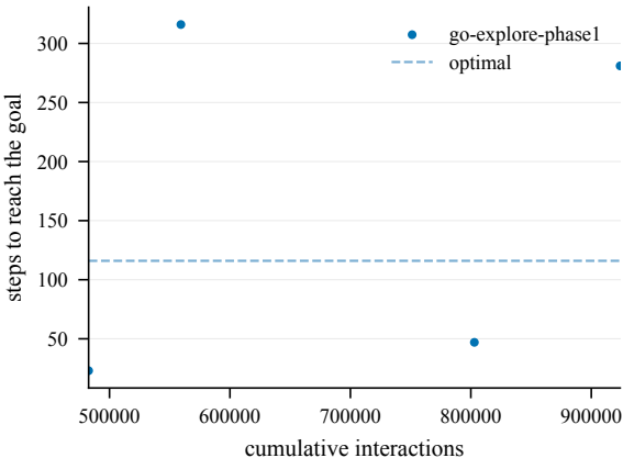
Steps to goal (train) -- Chambers2-100@4002
