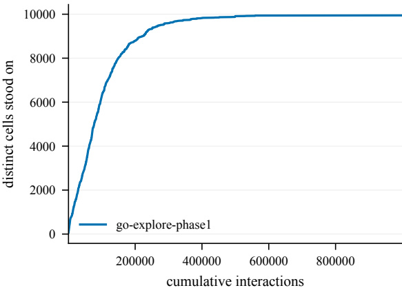
States discovered -- Chambers2-100@4002
