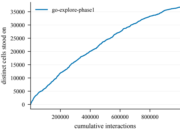
States discovered -- Chambers2-200@4001
