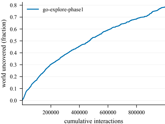
Cumulative coverage -- Chambers2-200@4002
