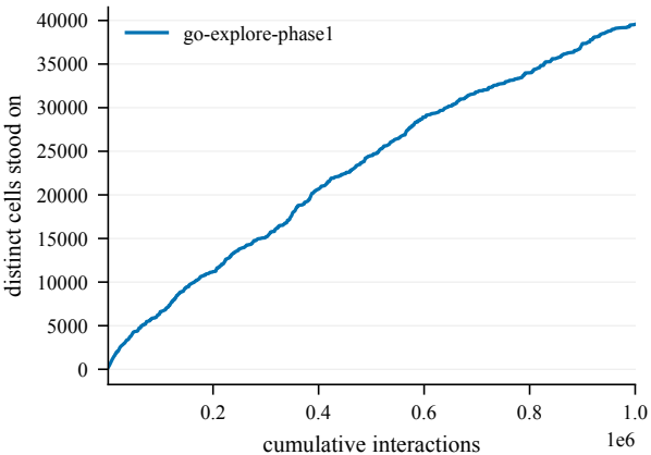
States discovered -- Chambers2-400@4000
