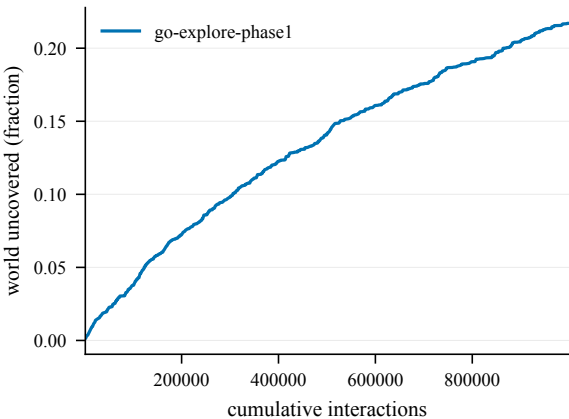
Cumulative coverage -- Chambers2-400@4002
