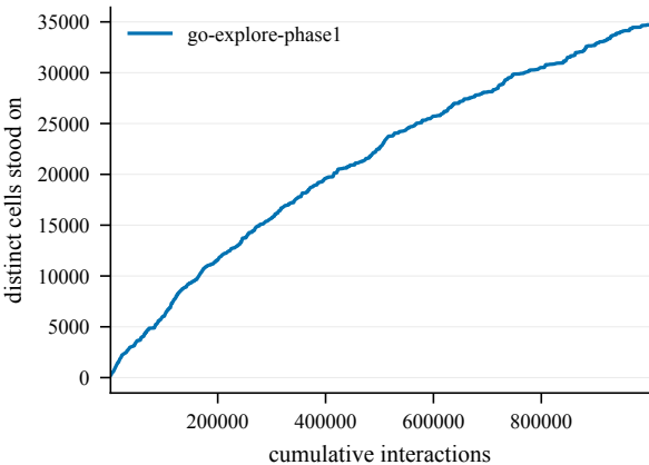
States discovered -- Chambers2-400@4002
