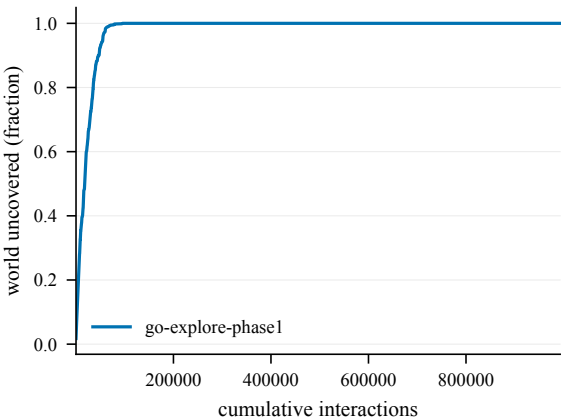
Cumulative coverage -- Chambers2-50@4000
