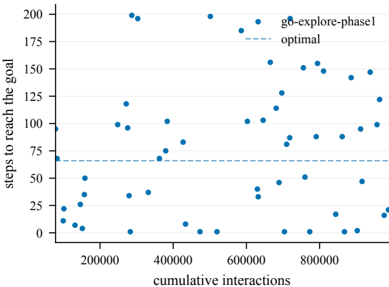
Steps to goal (train) -- Chambers2-50@4000
