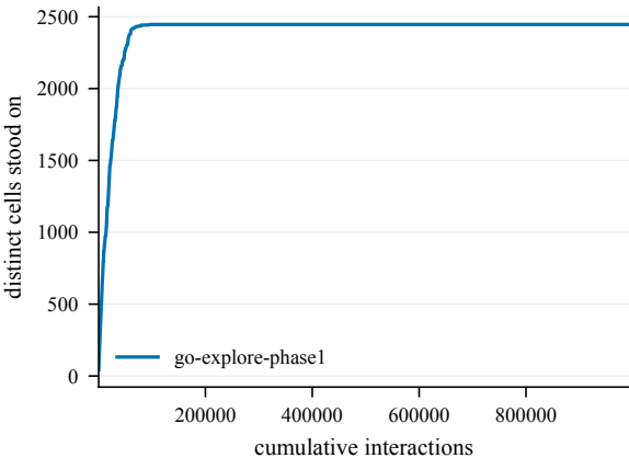
States discovered -- Chambers2-50@4000
