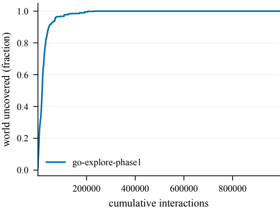
Cumulative coverage -- Chambers2-50@4001
