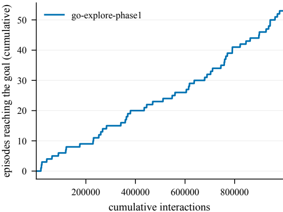
Goal reached -- Chambers2-50@4002
