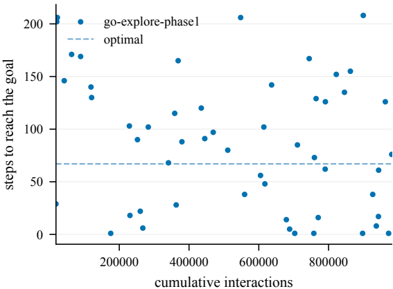
Steps to goal (train) -- Chambers2-50@4002
