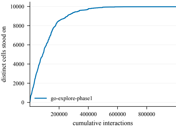
States discovered -- Decoys0-100@4000
