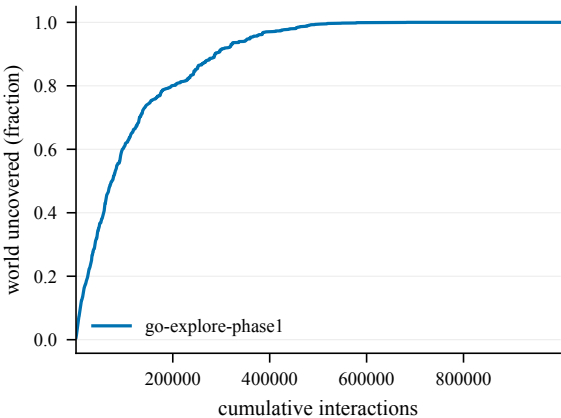
Cumulative coverage -- Decoys0-100@4001
