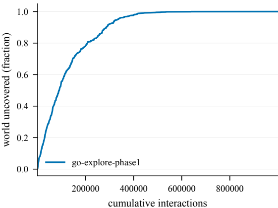
Cumulative coverage -- Decoys0-100@4002
