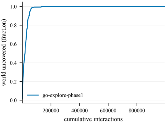
Cumulative coverage -- Decoys0-50@4002
