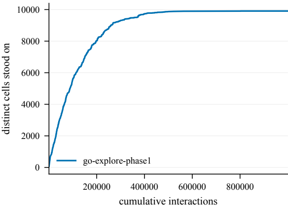
States discovered -- Decoys1-100@4000
