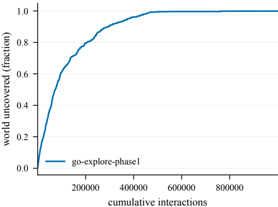
Cumulative coverage -- Decoys1-100@4001
