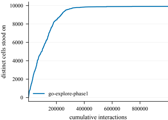
States discovered -- Decoys1-100@4002
