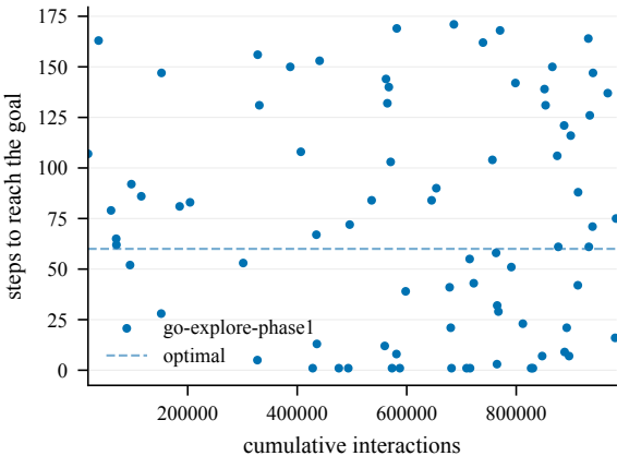
Steps to goal (train) -- Decoys1-50@4001
