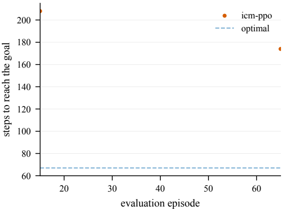
Steps to goal (eval) -- Decoys1-50@4002
