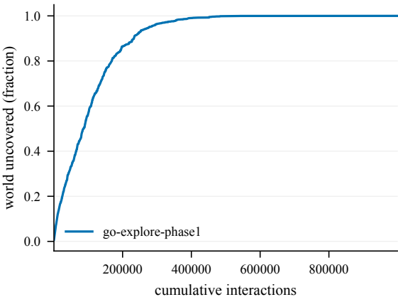
Cumulative coverage -- Decoys2-100@4001
