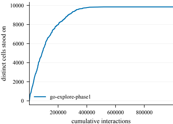
States discovered -- Decoys2-100@4002
