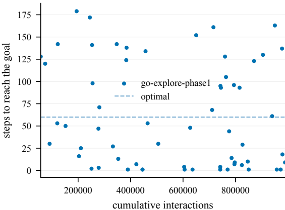
Steps to goal (train) -- Decoys2-50@4001
