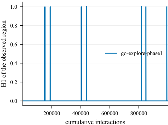
Discovered topology -- Decoys4-100@4001
