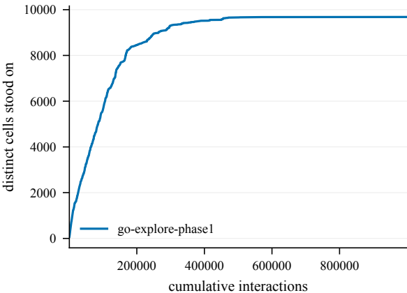
States discovered -- Decoys4-100@4001
