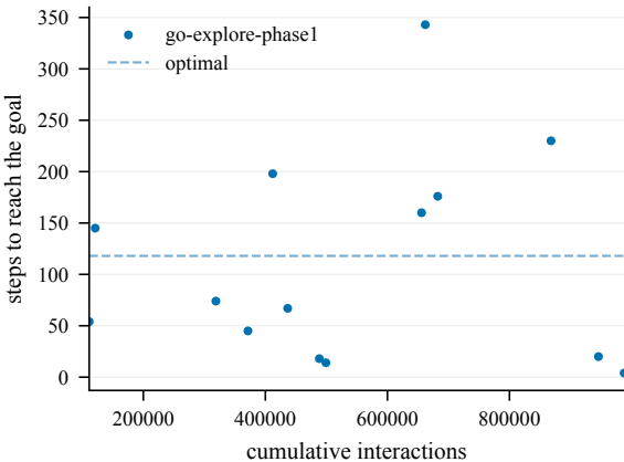
Steps to goal (train) -- Decoys4-100@4002
