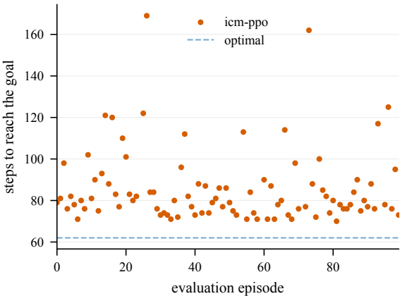
Steps to goal (eval) -- Decoys4-50@4001
