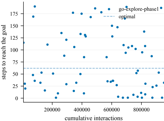
Steps to goal (train) -- Decoys4-50@4001
