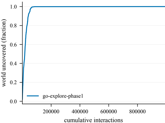
Cumulative coverage -- Decoys4-50@4002
