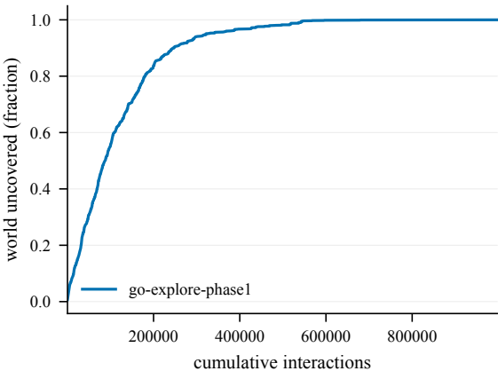
Cumulative coverage -- Decoys8-100@4001
