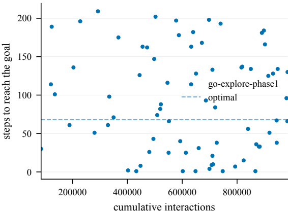
Steps to goal (train) -- Decoys8-50@4000
