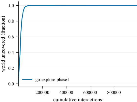
Cumulative coverage -- Decoys8-50@4001
