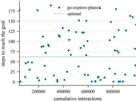
Steps to goal (train) -- Decoys8-50@4001
