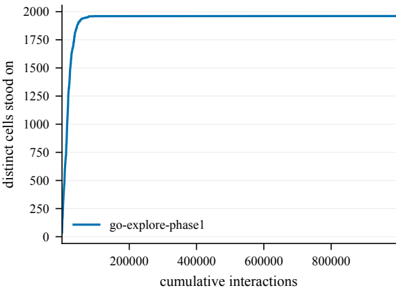
States discovered -- Decoys8-50@4001
