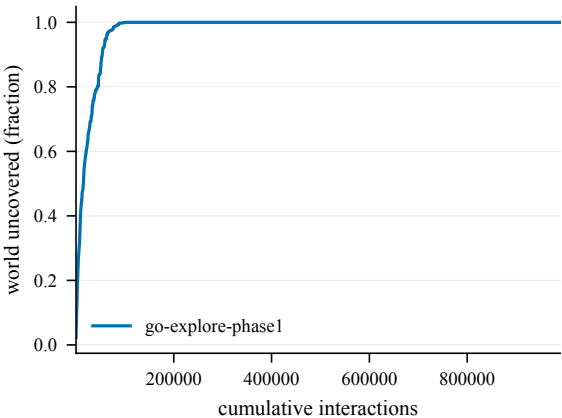
Cumulative coverage -- Decoys8-50@4002
