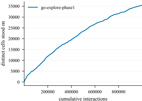
States discovered -- Dilution-200@4001
