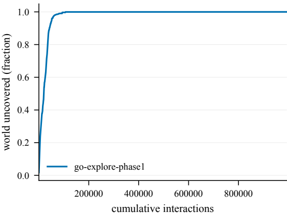
Cumulative coverage -- Dilution-50@4000
