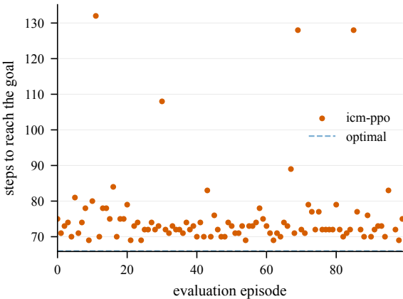
Steps to goal (eval) -- Dilution-50@4000
