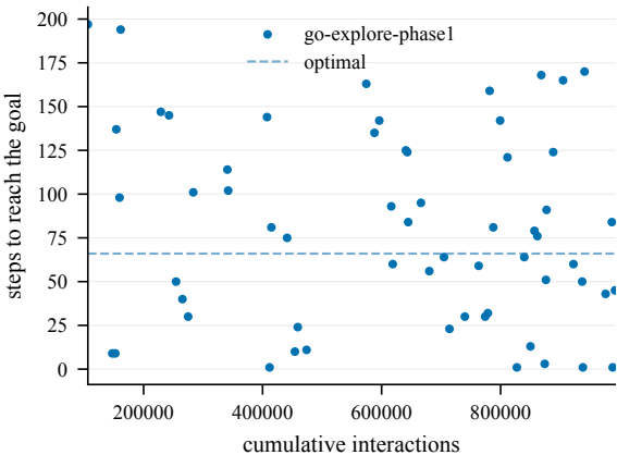
Steps to goal (train) -- Dilution-50@4000
