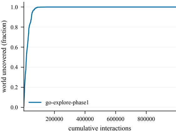
Cumulative coverage -- Dilution-50@4001
