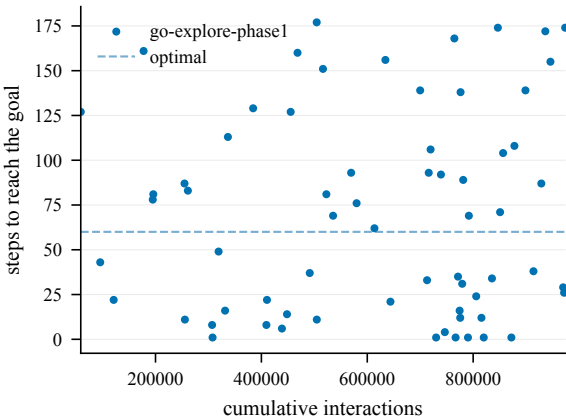
Steps to goal (train) -- Dilution-50@4001
