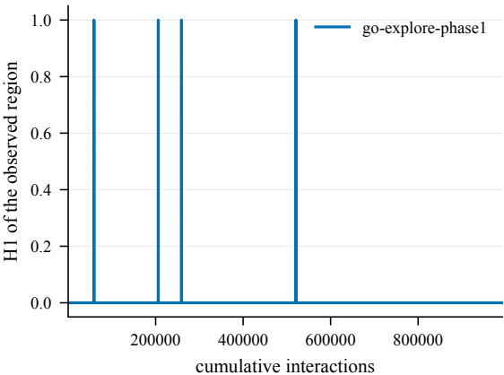
Discovered topology -- Dilution-50@4002
